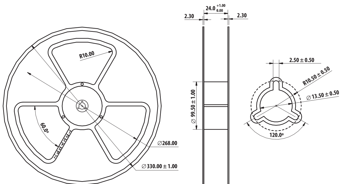
Figure 21. Reel dimensions
